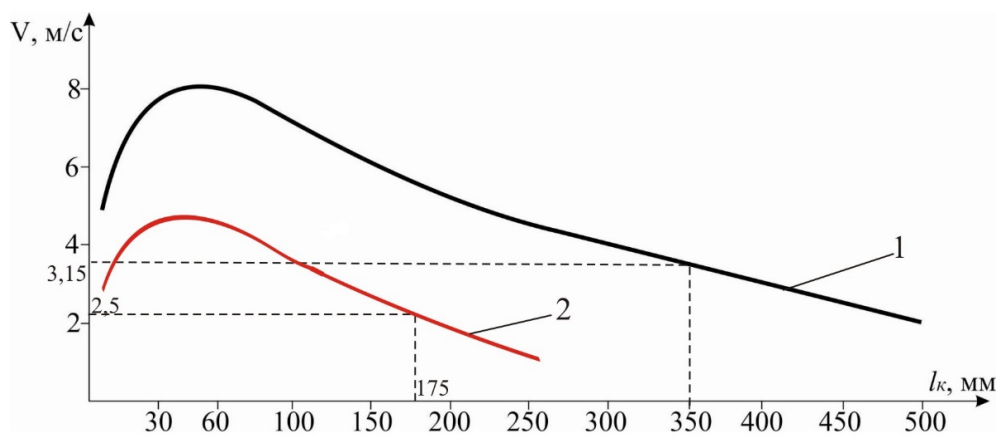
1 - inclined conveyor (according to [1]) and 2 - steeply inclined conveyor (SIC)
